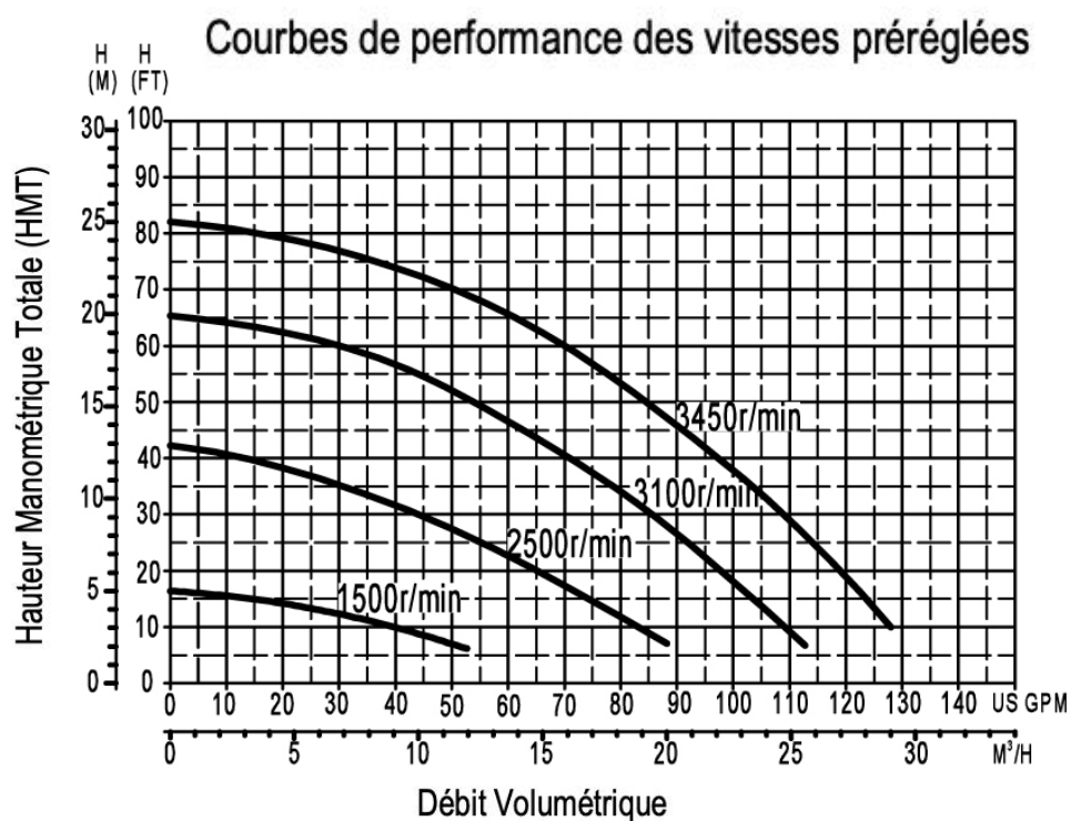
BDXTVAR200 2.0HP Courbes de performance
