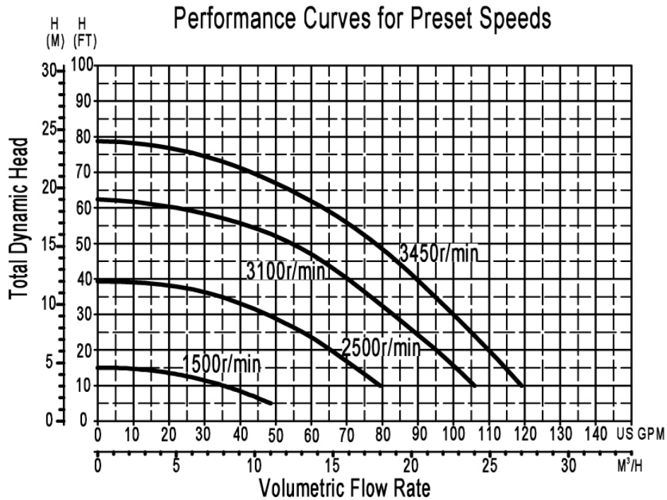
BDXTVAR150 1.5HP Performance Curves
