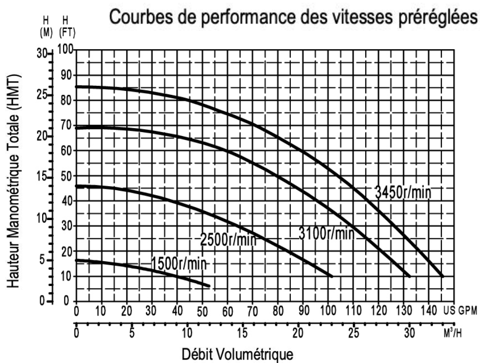
BDXTVAR300 3.0HP Courbes de performance
