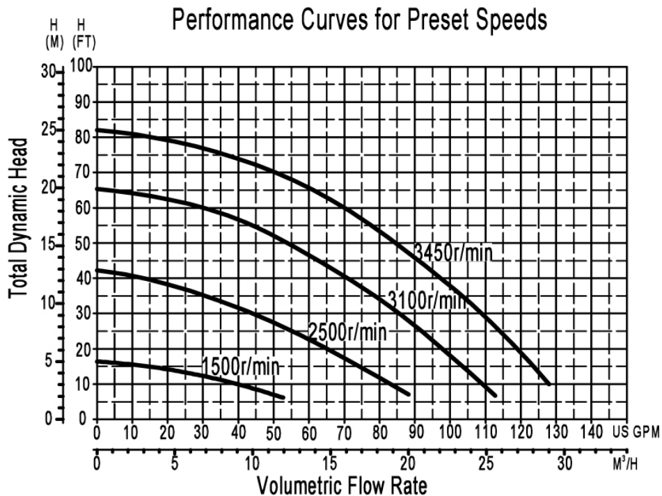
BDXTVAR200 2.0HP Performance Curves
