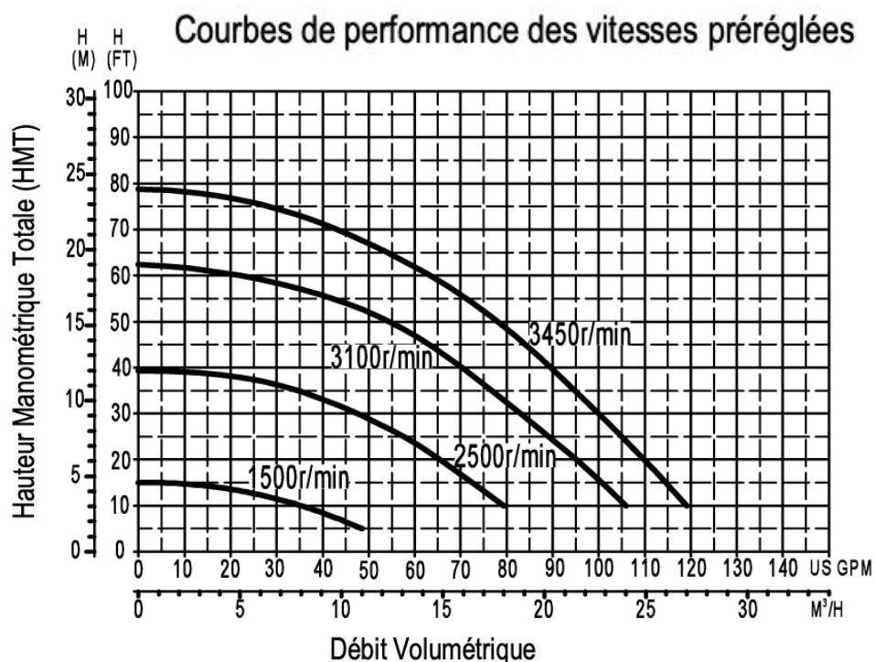
BDXTVAR150 1.5HP Courbes de performance
