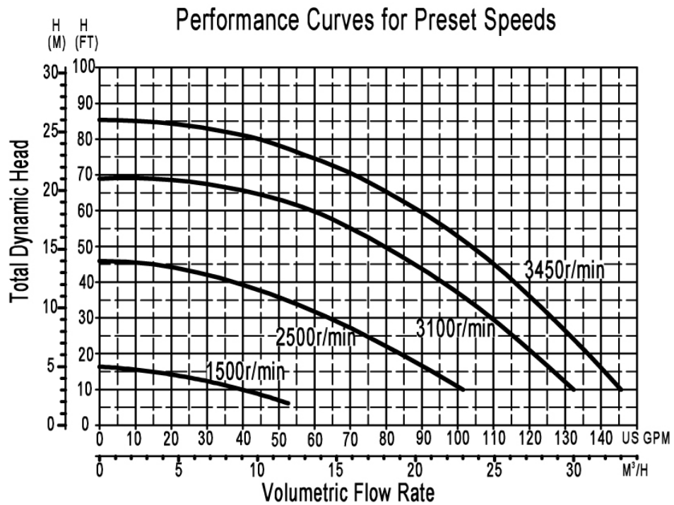
BDXTVAR300 3.0HP Performance Curves
