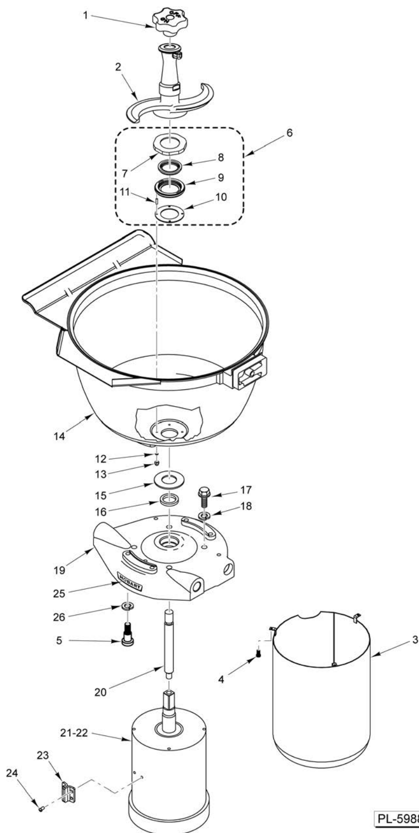
BOWL AND MOTOR ASSEMBLY (PREVIOUS CONSTRUCTION)
