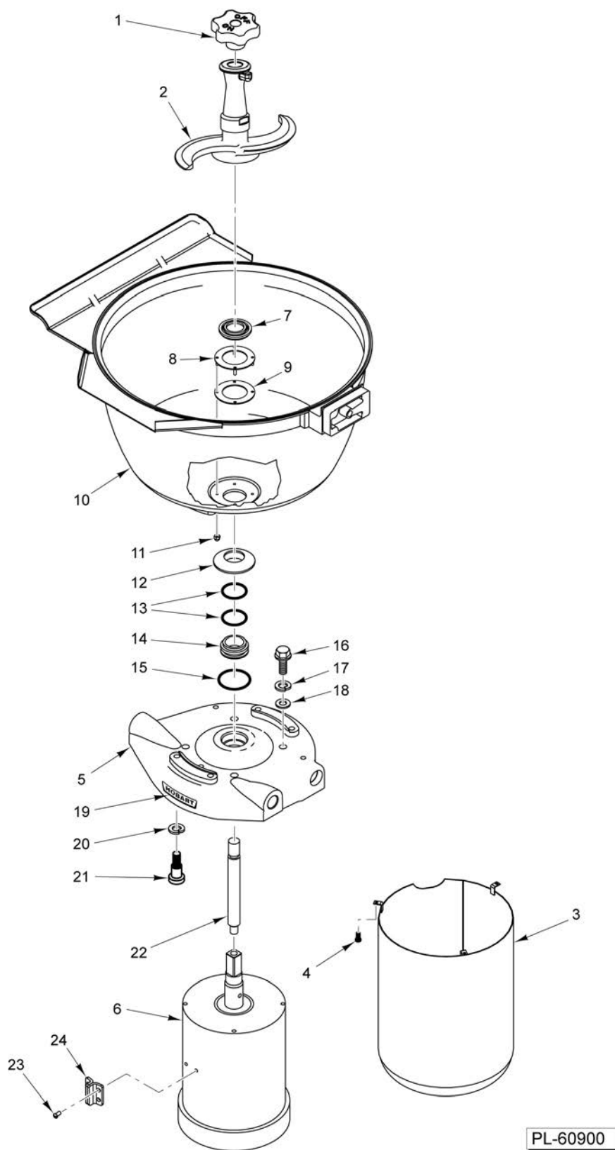
BOWL AND MOTOR ASSEMBLY (CURRENT CONSTRUCTION)
