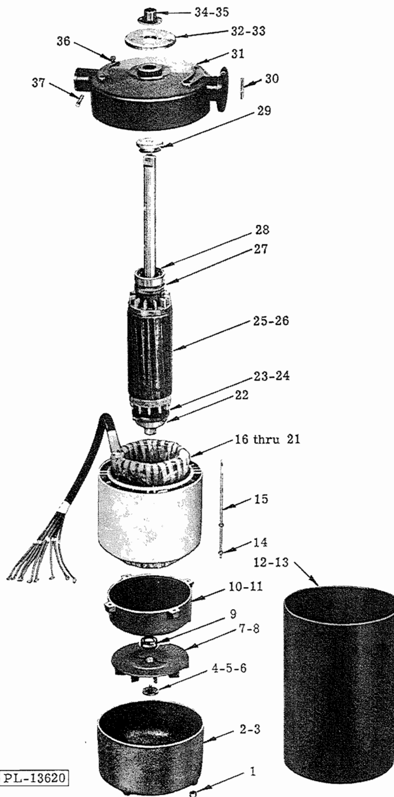
MOTOR UNIT (PRIOR TO SERIAL NO. 76 U-20 000)
