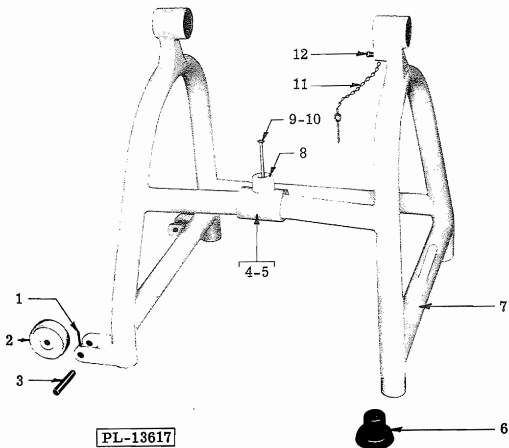
CHASSIS UNIT
