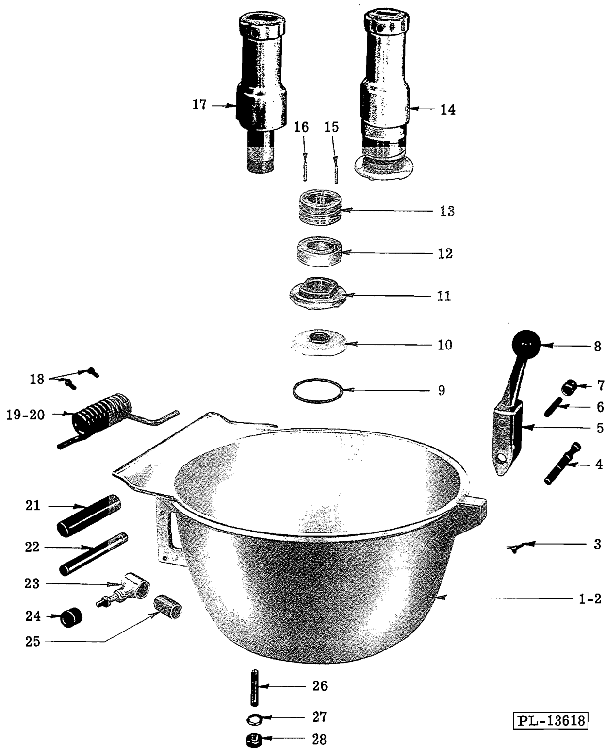
BOWL UNIT
